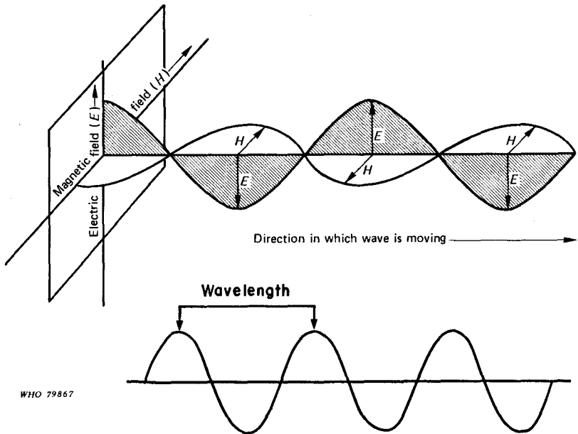
Fig. 1. An electromagnetic monochromatic wave. Electromagnetic waves consist of electrical and magnetic forces which move in consistent wave-like patterns at right angles to one another.
