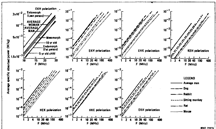
Fig. 11. Average specific absorbed power in ellipsoidal models of man and test animals; incident power density 1 \text{ mW/cm}^2 (From: National Health and Welfare, Canada (1977) based on Rowe et al., 1973).
