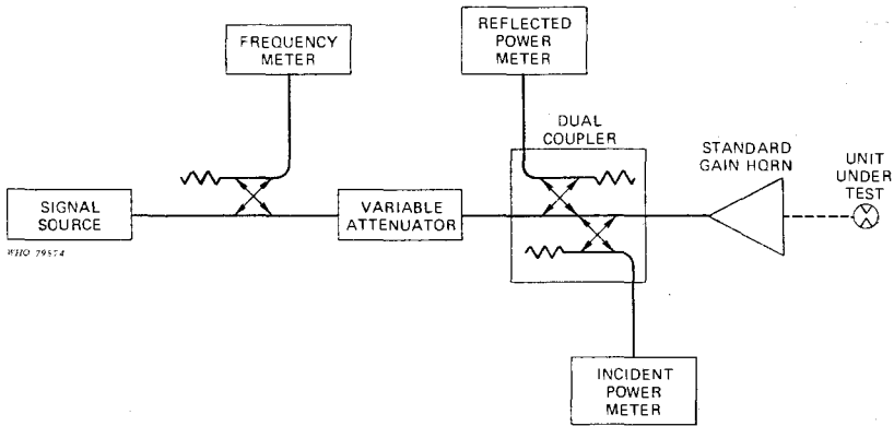
Fig. 9. Diagram of the basic experimental arrangement required for the free space standard field method.
