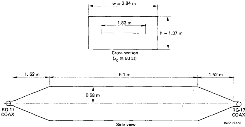
Fig. 10. A type of TEM transmission cell used at the US National Bureau of Standards for calibrating hazard meters and for measuring the susceptibility of electronic equipment to EM fields. Such cells can also be used as exposure chambers for studying biological effects. This cell was designed for an upper frequency limit of about 500 MHz.
