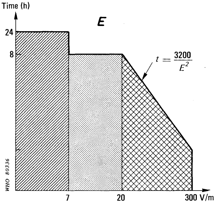
Fig. 20. Permissible limits for occupational ( \leq 10 -h) and general public (24-h) exposure to radiofrequency radiation (10–300 MHz) in Poland.
