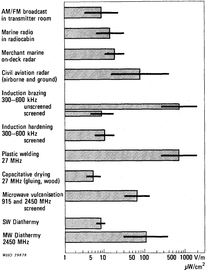
Fig. 22. Field strengths typically occurring in the vicinity of industrial equipment and work places.
