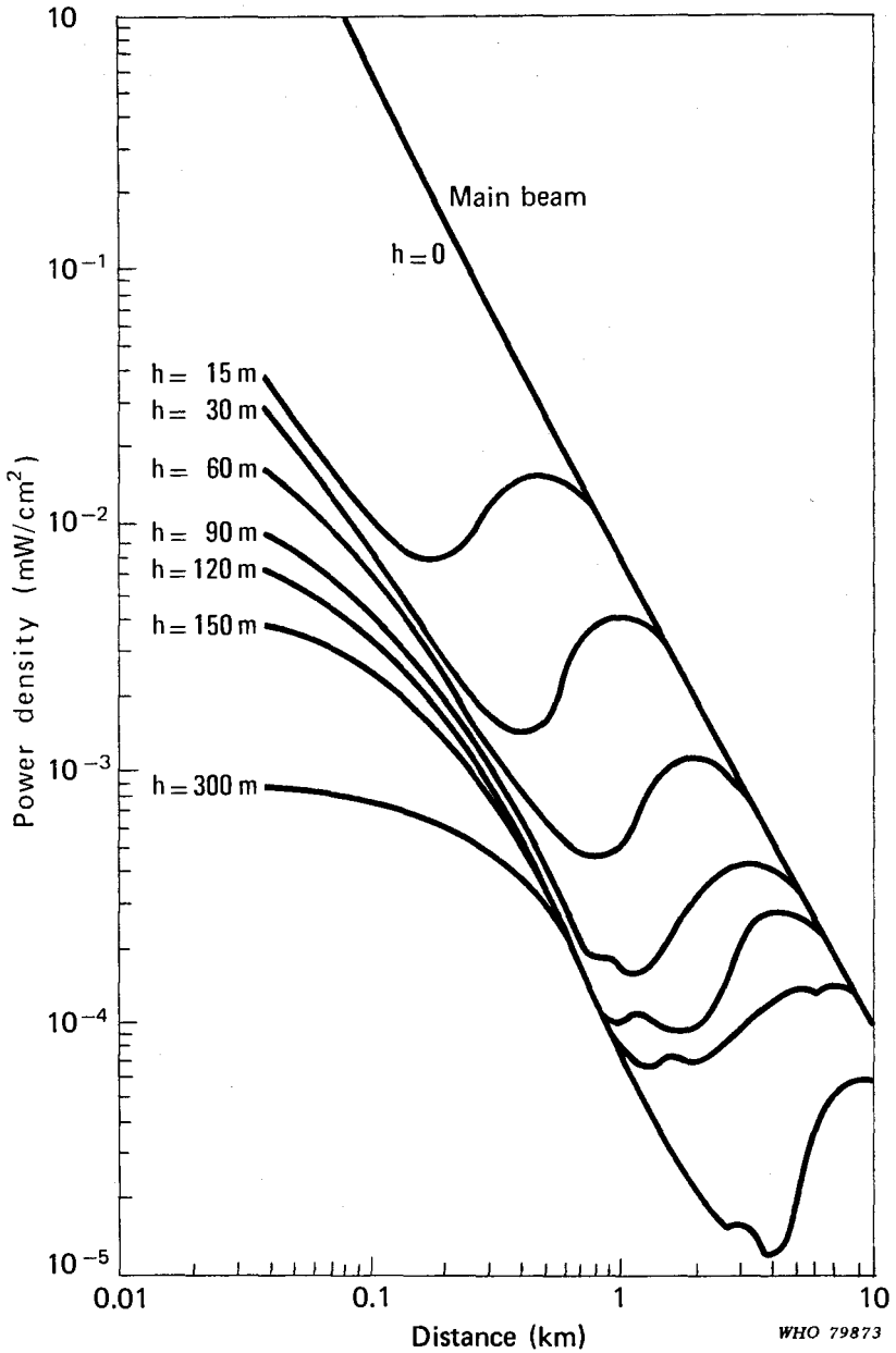
Fig. 8. Power density versus distance at various heights for a TV station with ERP equal to 1 \text{ mW}/\text{cm}^2 (From: National Health and Welfare, Canada, 1977).
