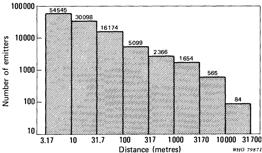
Fig. 6. Microwave sources in the USA in 1973, capable of producing a power density equal to or greater than 0.1 \text{ mW/cm}^2 (From: National Health and Welfare, Canada (1977) based on Rowe et al., 1973).
