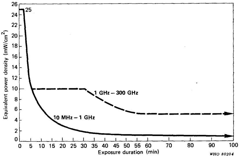
Fig. 17. Occupational exposure limits for workers exposed to microwaves in the frequency range 10 MHz—300 GHz (From: National Health and Welfare, Canada, 1979).
