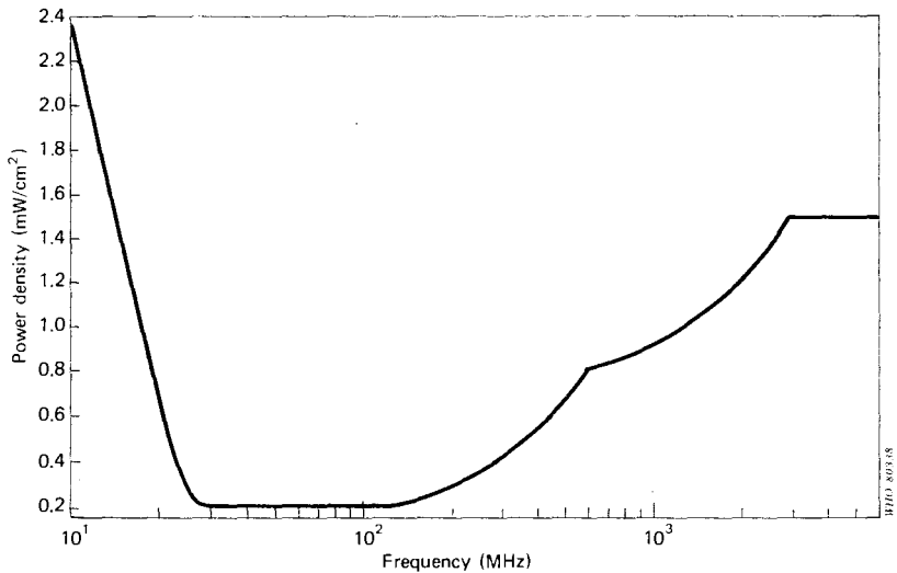
Fig. 18. Maximum permissible exposure limits according to an Australian draft proposal (From: Cornelius & Viglione, 1979).
