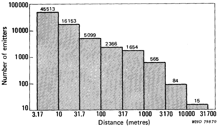
Fig. 5. Microwave sources in the USA in 1973, capable of producing a power density equal to or greater than 1 mW/cm 2 (From: National Health and Welfare, Canada (1977) based on Rowe et al., 1973).
