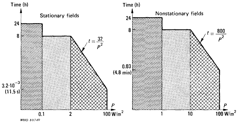
Fig. 16. Permissible limits for occupational ( \leq 10 -h) and general public (24-h) exposure to microwave radiation (0.3—300 GHz) in Poland.
