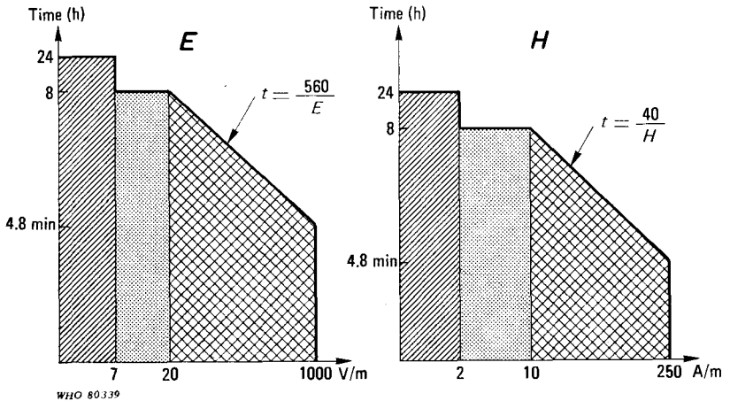
Fig. 21. Permissible limits for occupational ( \leq 10 -h) and general public (24-h) exposure to radiofrequency radiation (0.1–10 MHz) in Poland.
